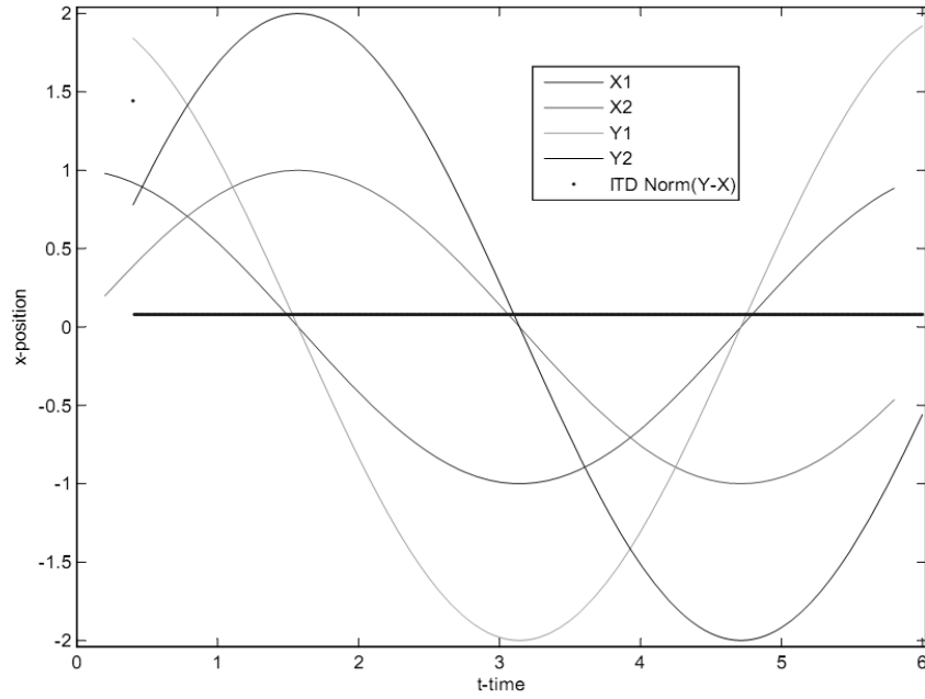
Figure 6. Approximate Solutions provided by the Euler Method with h = 0.01
