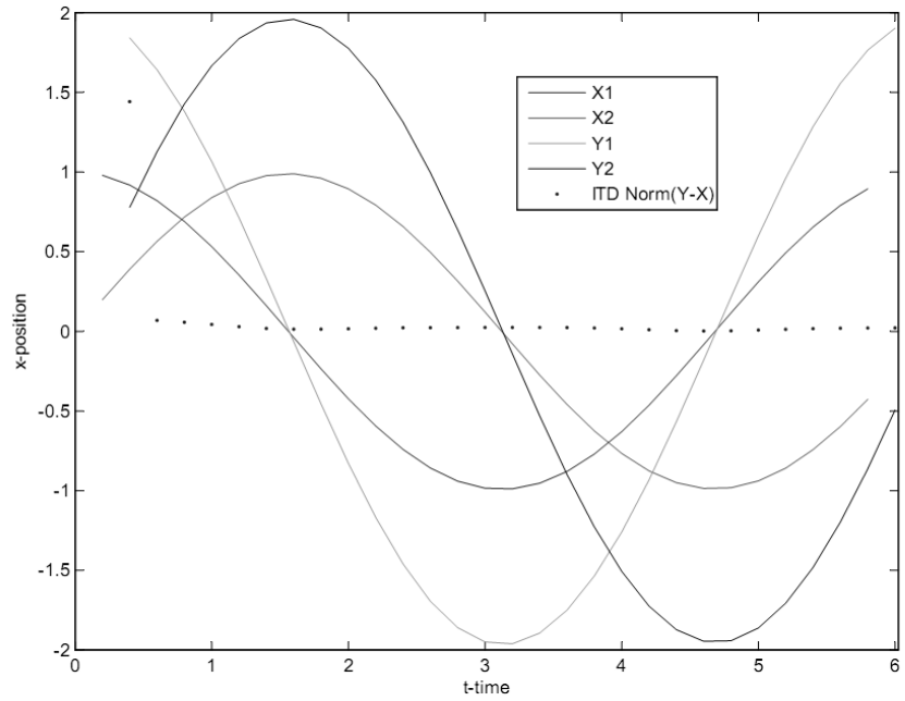
Figure 2. Approximate Solutions provided by the Improved Euler Method with h = 0.2
