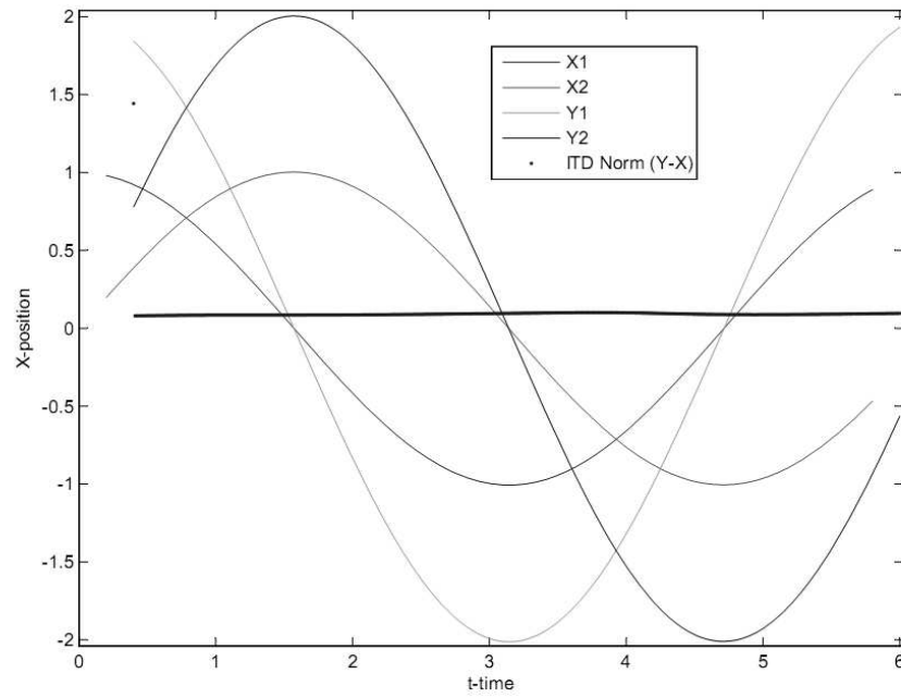
Figure 6. Approximate Solutions provided by the Euler Method with h = 0.01
