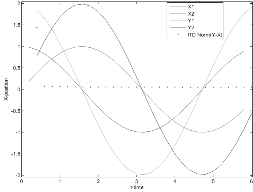
Figure 1. Approximate Solutions provided by the Runge-Kutta Method with h = 0.2
