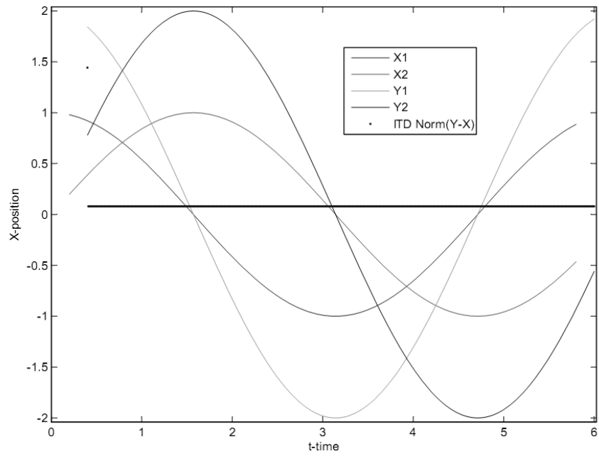
Figure 4. Approximate Solutions provided by the Runge-Kutta Method with h = 0.01
