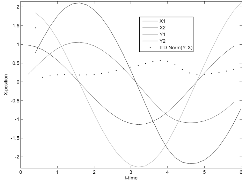
Figure 4. Approximate Solutions provided by the Runge-Kutta Method with h = 0.01
