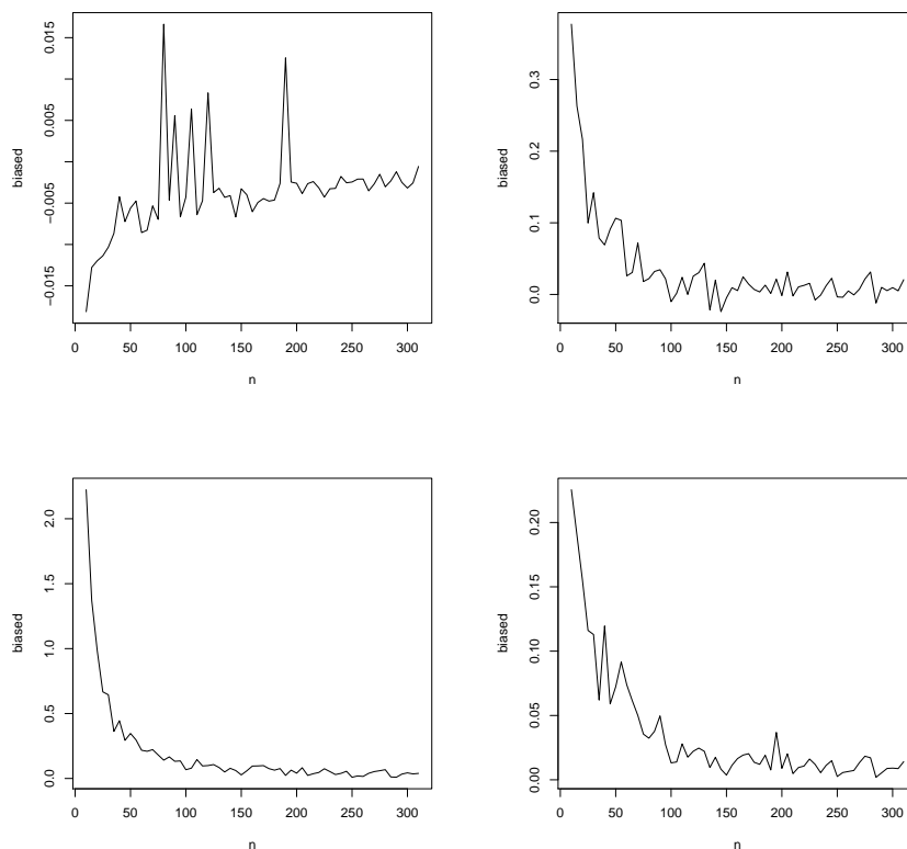
Figure 3. Bias_\alpha(n) (top left), Bias_\lambda(n) (top right), Bias_a(n) (bottom left) and Bias_b(n) (bottom right) versus n = 10, 15, 20, \dots, 320 .
