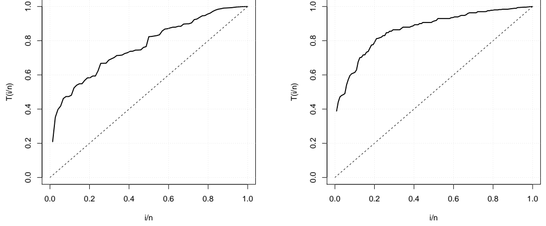
Figure 6. TTT-plot for the first data set (left figure) and for the second data set (right figure).
